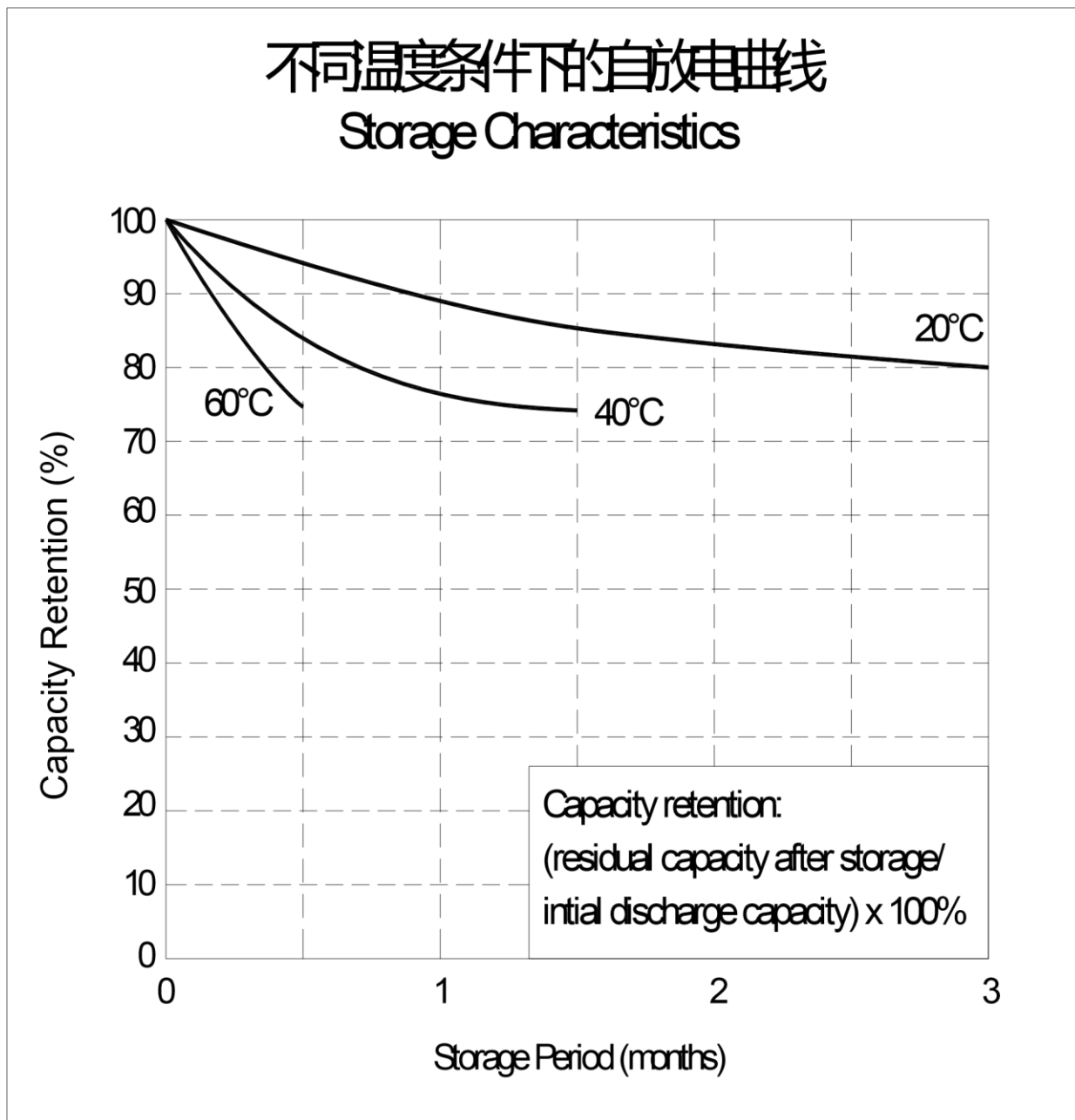
Fig. 4 Storage Characteristics
